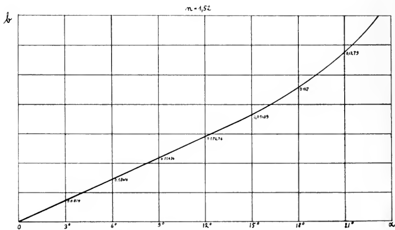
FIG. 2. The relation between the displacement and the angle of incidence.
